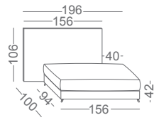
_pouf 156 con pannello _ottoman 156 with back panel
