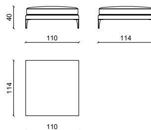
ISOLA / ISLAND 110
