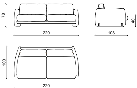
DIVANO / SOFA 220
