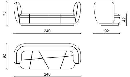
DIVANO / SOFA 240
